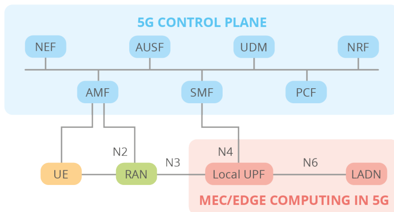
Local UPF support with local area data network (LADN)
